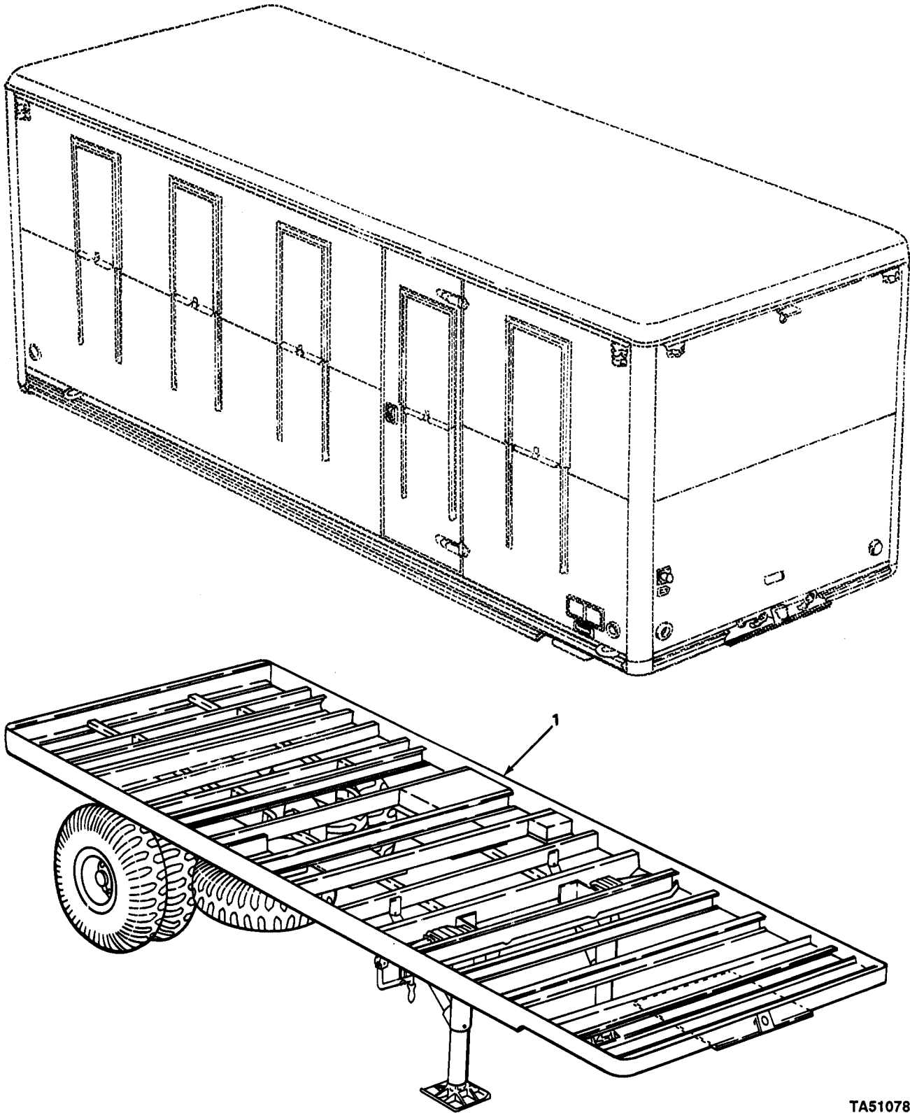
FIGURE 27. TRAILER FRAME.
