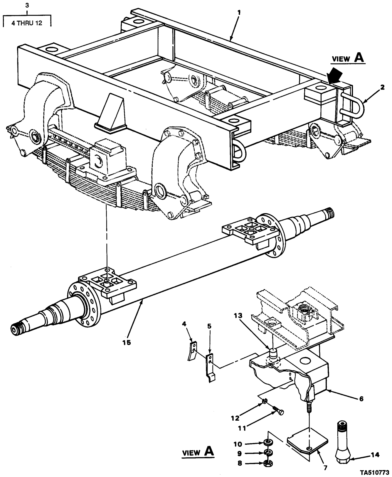
FIGURE 13. AXLE.
