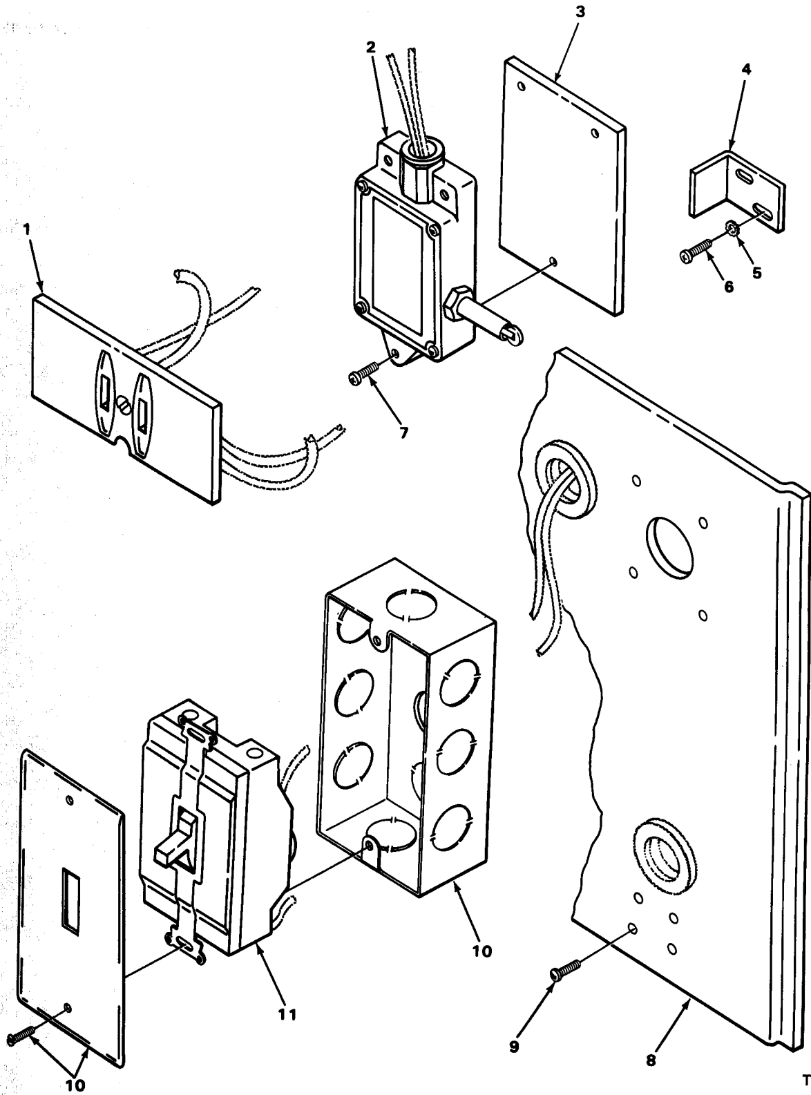
FIGURE 1. LIGHT SWITCHES.
