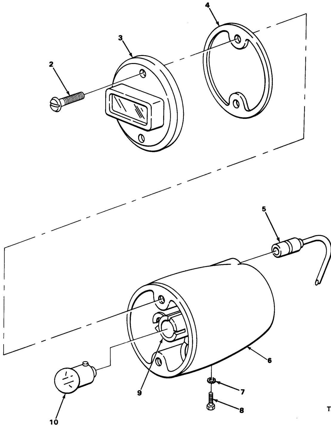
FIGURE 5. BLACKOUT LIGHT
