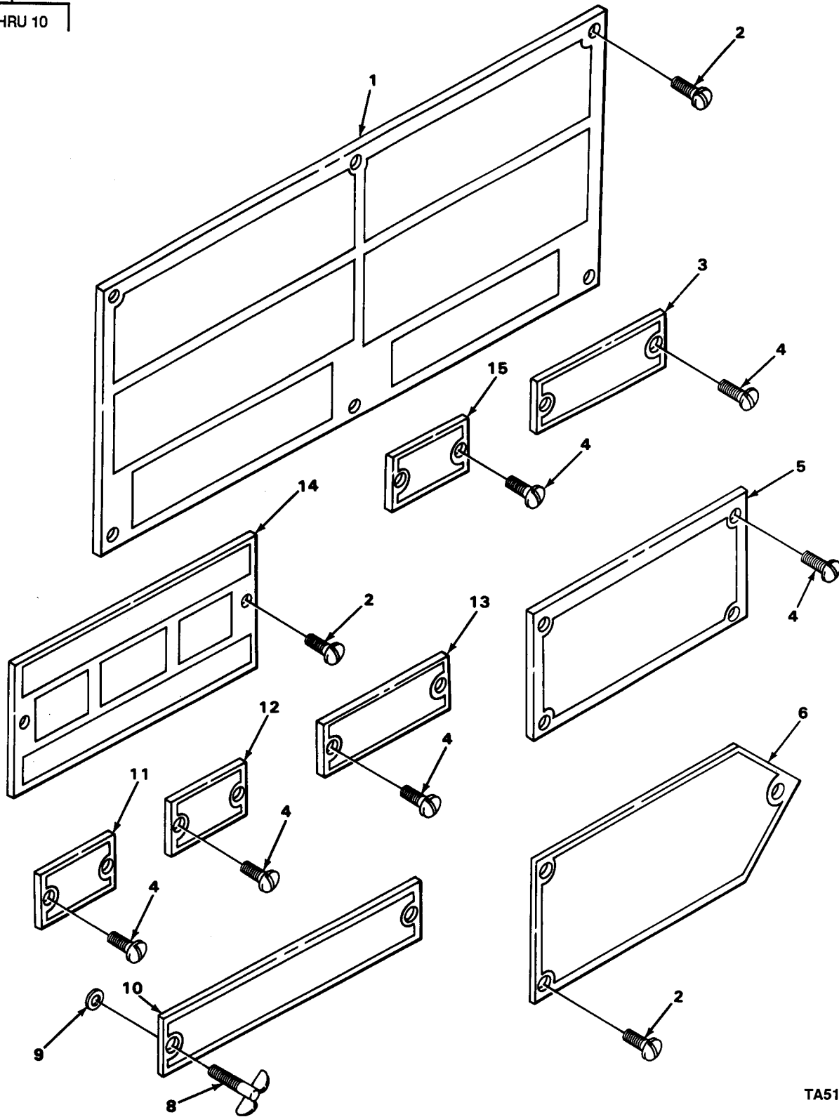
FIGURE 47. DATA PLATES.
