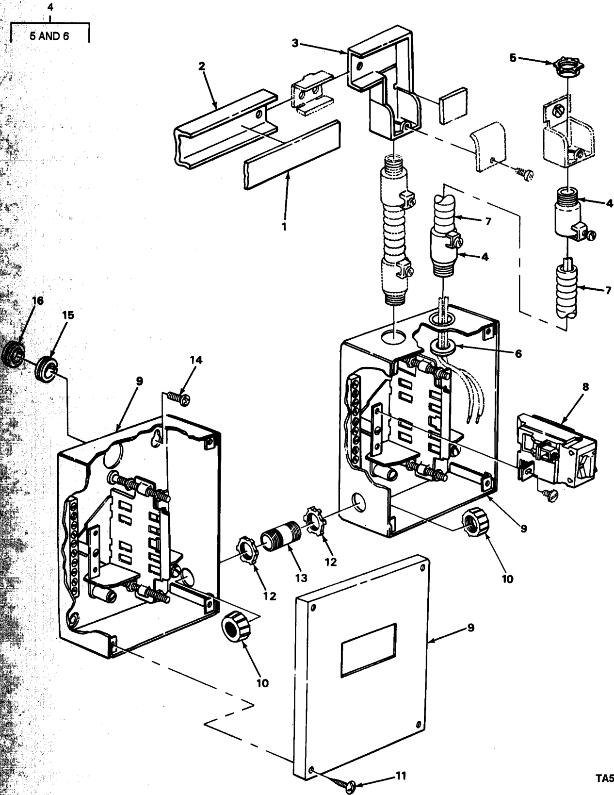
FIGURE 2. JUNCTION BOXES.
