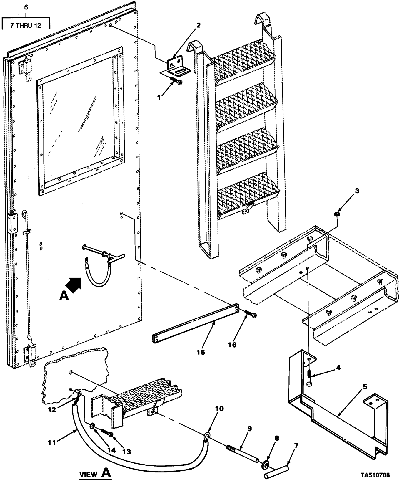
FIGURE 28. LADDER AND MOUNTING PARTS.
