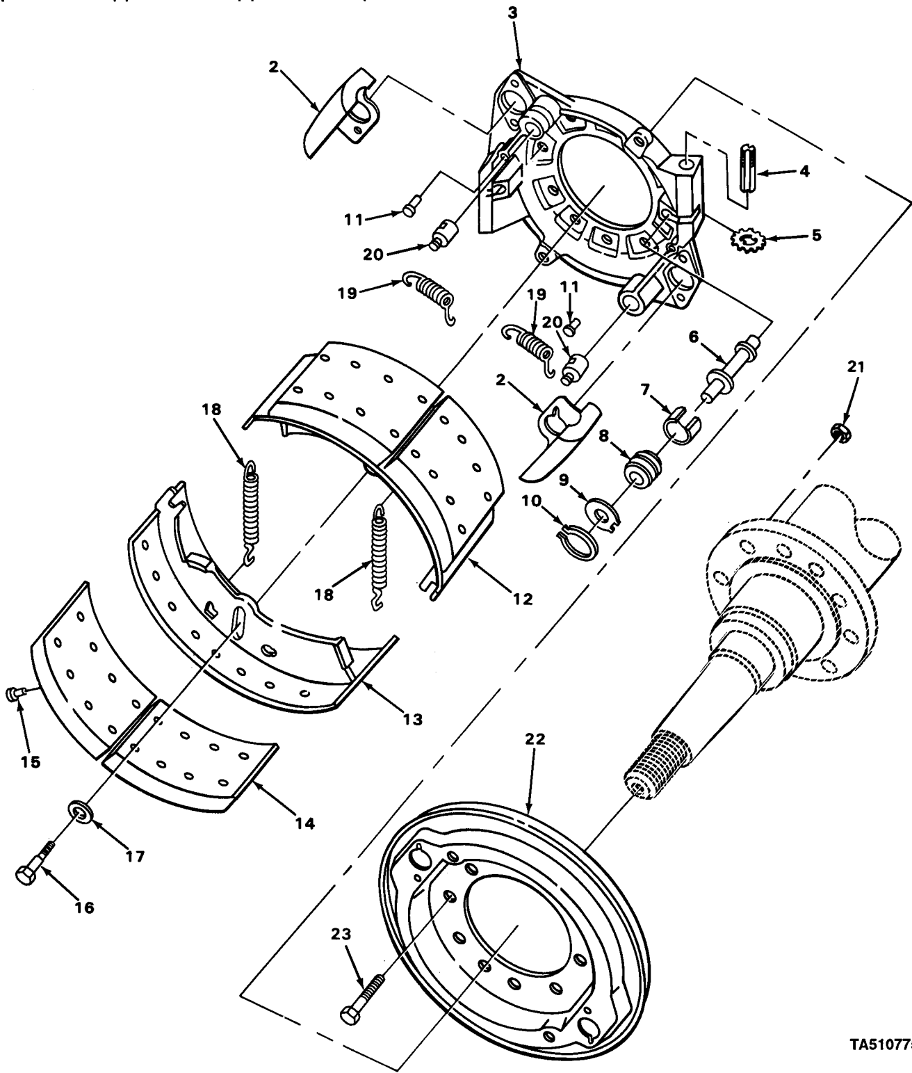
FIGURE 15. BRAKE AND SPIDER ASSEMBLY.
