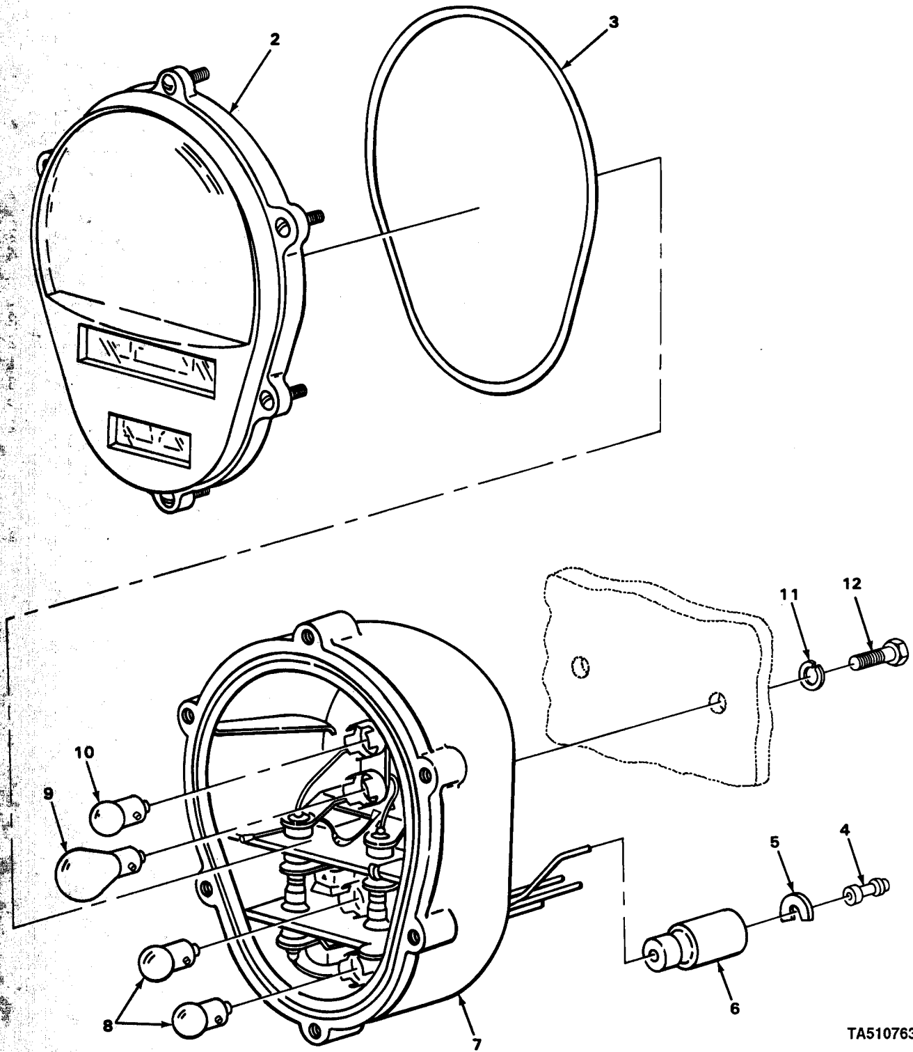
FIGURE 3. COMPOSITE LIGHT.
