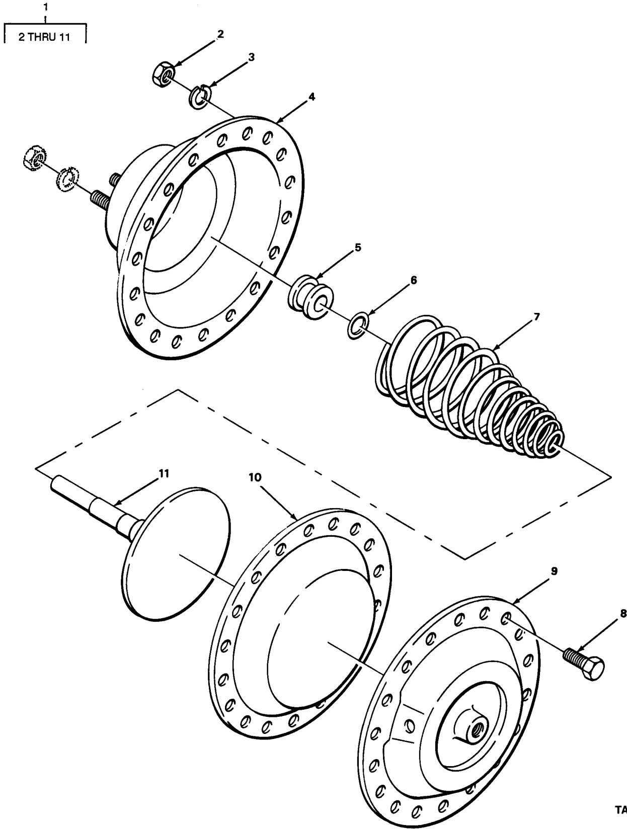
FIGURE 21. AIR CHAMBER.
