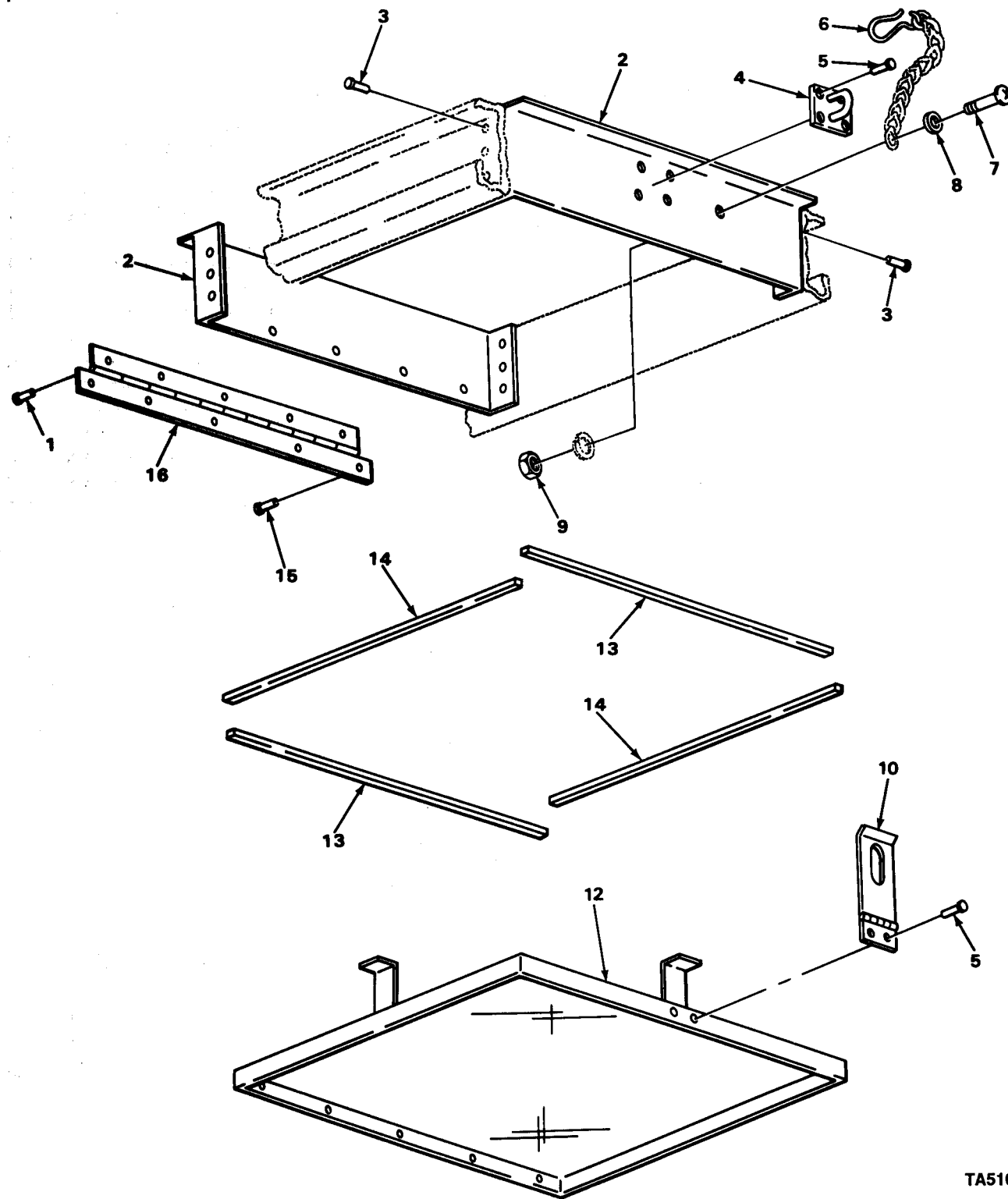
FIGURE 42. CABLE STORAGE BOX.
