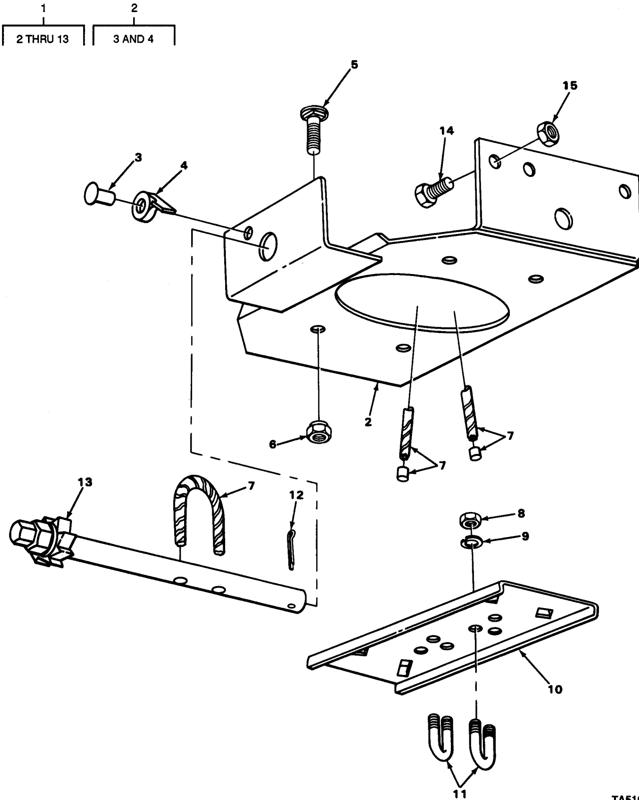
FIGURE 29. TIRE CARRIER.
