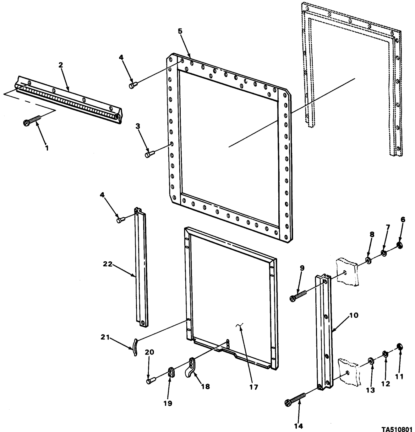
FIGURE 41. WINDOW AND BLACKOUT PANEL (EXTERIOR VIEW).
